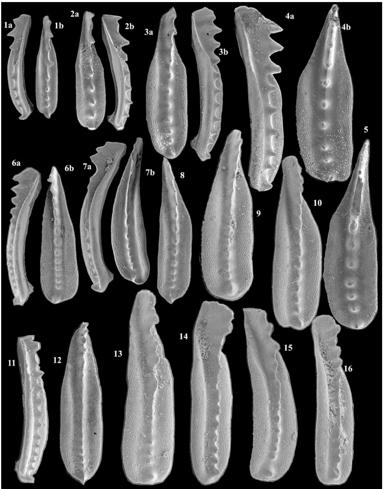
Figure 7 Key conodonts from the Tiegiao and Penglaitan sections. All specimens are SEM photos magnified the same amount (for scale specimen 9 is exactly 1 mm in length). Letters a and b designate different views of the same specimen. 1, 6–10, 13–16, Clarkina postbitteri hongshuiensis Henderson et al., 2002 showing the specimens with closely spaced and often fused denticles, especially in adult specimens. Specimens 1, 6, 8, 13–16 are from Bed 6i-upper and 7, 9, 10 are from Bed 6j at the Penglaitan Section. 2–5, Clarkina postbitteri postbitteri Mei and Wardlaw in Mei et al., 1994a showing the specimens with more widely spaced and consistently discrete denticles and abruptly narrowing anterior (top in figure) platform. All specimens are from Bed 6k at the Penglaitan Section. 11–12, Jinogondolella granti Mei and Wardlaw in Mei et al., 1994a from Bed 6h at the Tiegiao Section.
