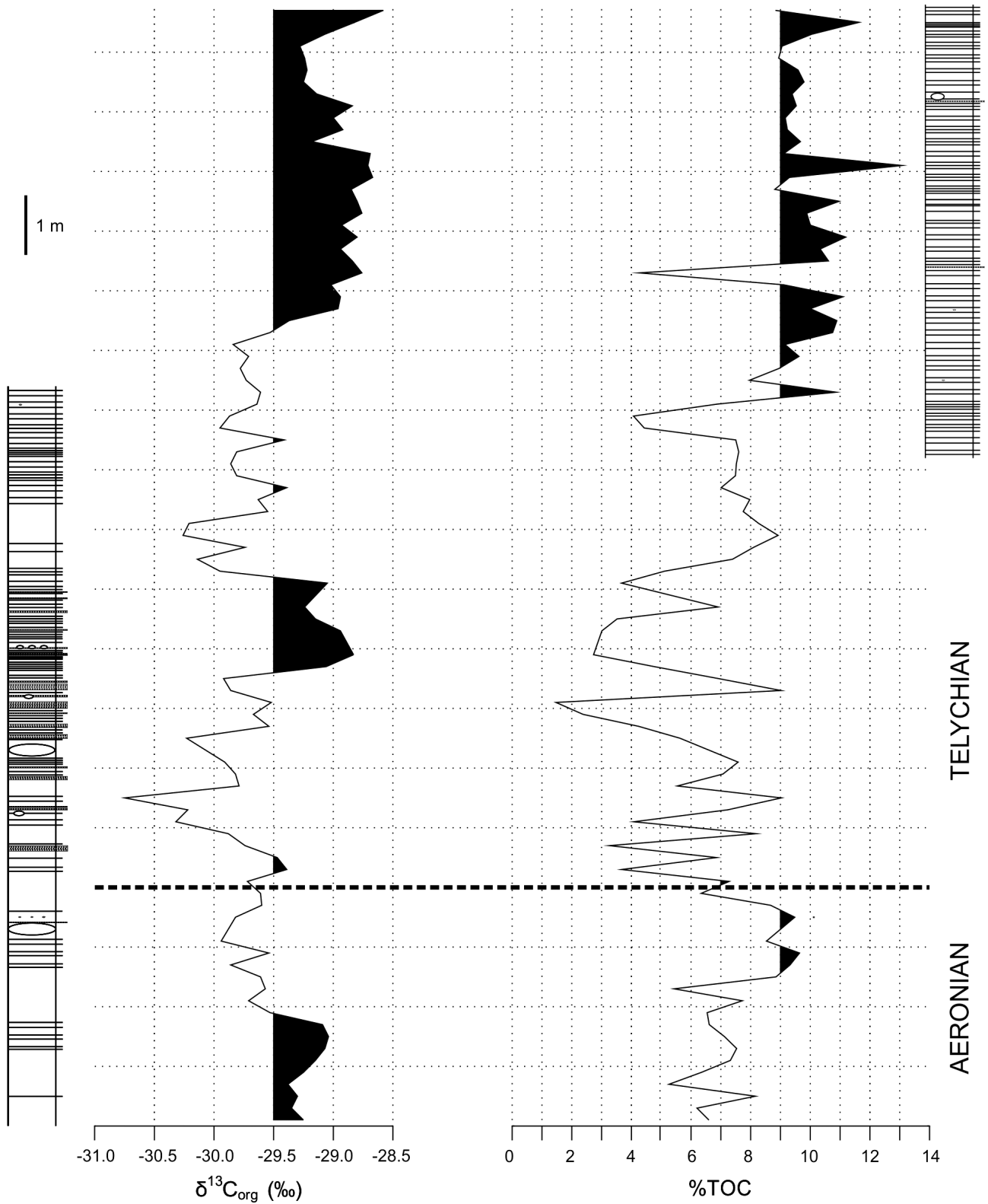
Figure 13. The \delta^{13}C_{org} and TOC records through El Pintado sections 1 and 5. Shading is used to highlight higher ( i.e. less negative) \delta^{13}C_{org} (above -29.5\text{‰} ) and TOC (above 9%) values. See Fig. 9 for explanation of lithological symbols used.
